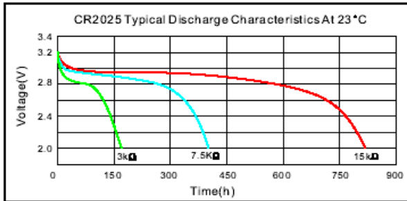
Discharge Characteristics on Load
