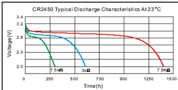
Discharge Characteristics on Load
