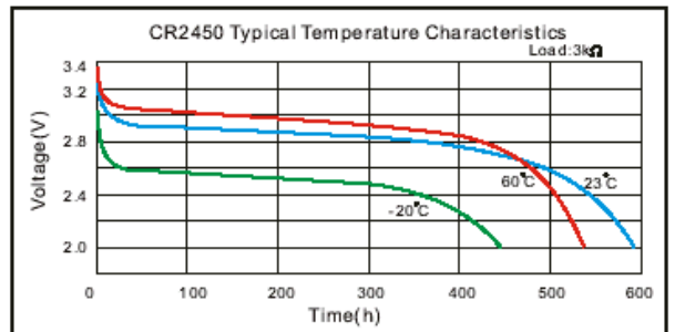
Discharge Characteristics on Temperature
